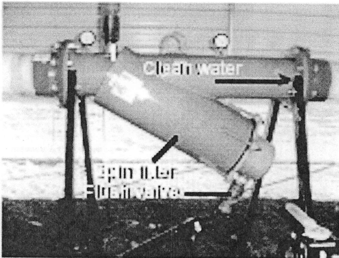
Figure 4. Spin filter
