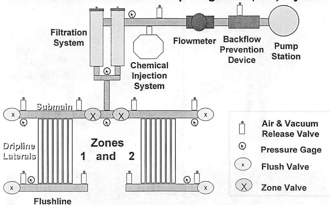
Figure 2. Schematic of a subsurface drip irrigation system.
