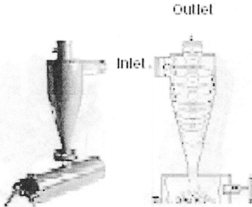
Figure 5. Schematic diagram and example sand separator.
