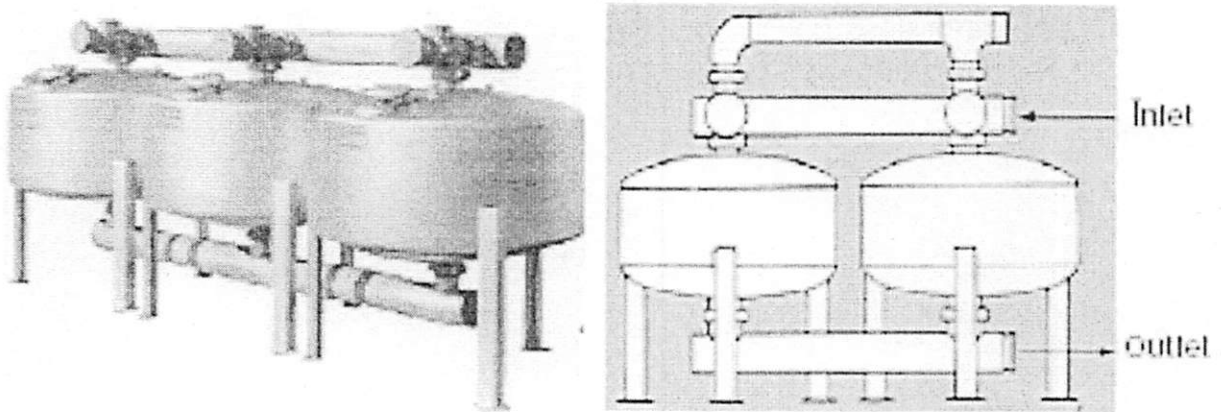
Figure 6. Schematic diagram and example media filter.
