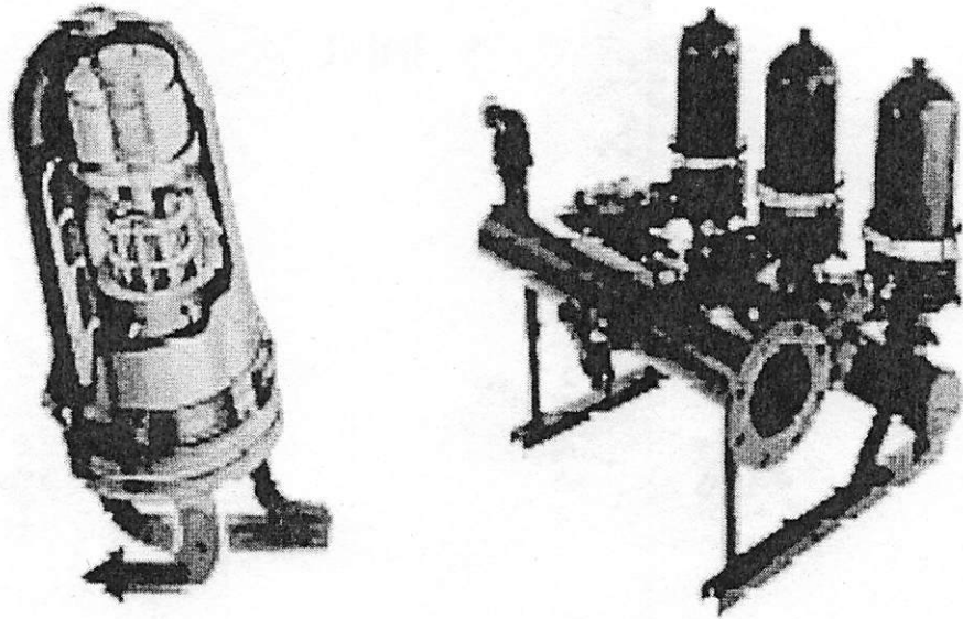
Figure 7. Schematic diagram and example disk filter.
