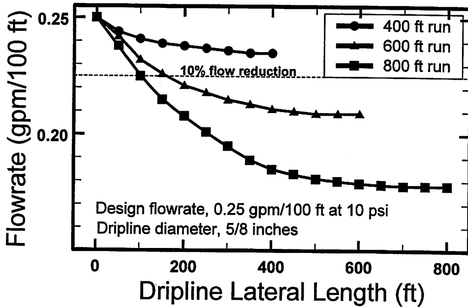
Figure 2. Calculated dripline flowrates on level slopes as affected by length of run. For this example dripline, only the 400 ft lateral length meets the desired criteria of maintaining flow variations less than 10%.
