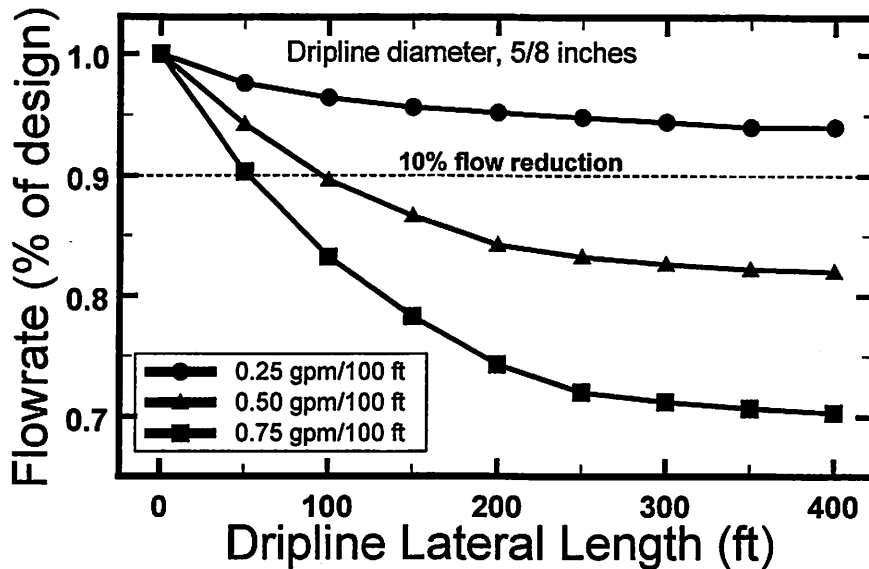
Figure 3. Calculated flowrates on level slopes as affected by dripline capacity. In this example only the 0.25 gpm/100 ft dripline capacity meets the desired criteria of maintaining flow variations less than 10%.
