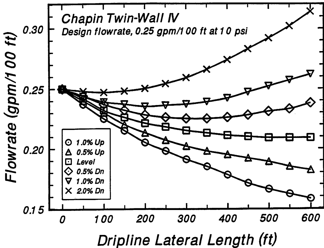
Figure 3. Calculated dripline flowrates as affected by slope. Data from Chapin Watermatics 1 .
