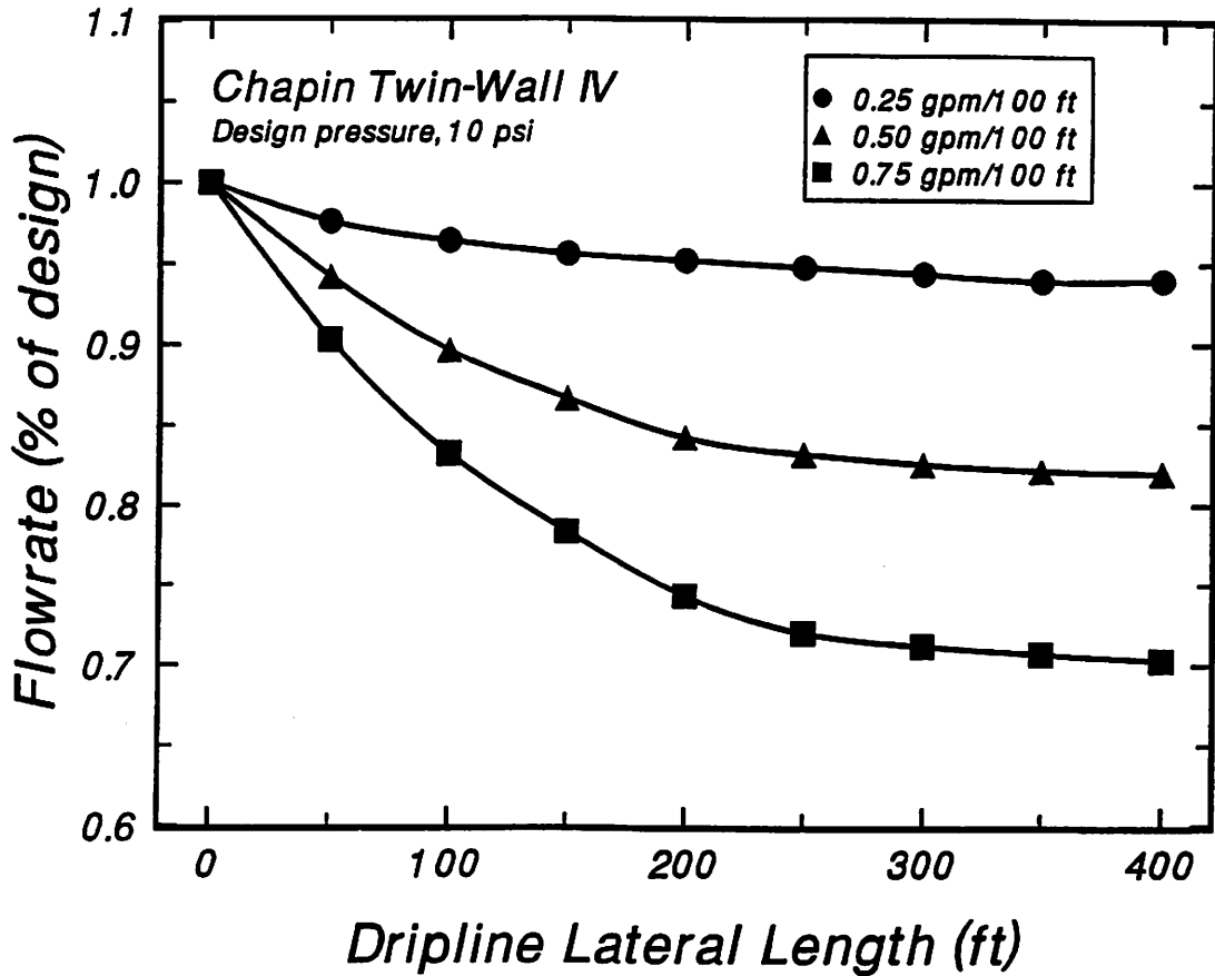
Figure 1. Calculated dripline flowrates on level slopes as affected by length of run. Data from Chapin Watermatics 1 .
