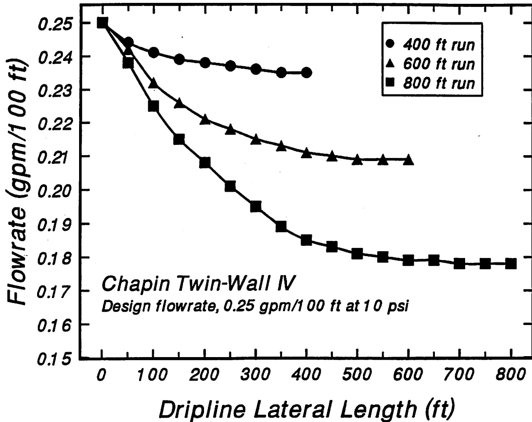
Figure 2. Calculated dripline flowrates on level slopes as affected by dripline capacity. Data from Chapin Watermatics 1 .
