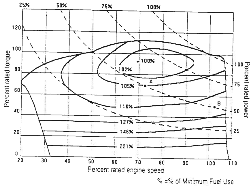
Figure 4: Example of an Engine Performance Curve.
