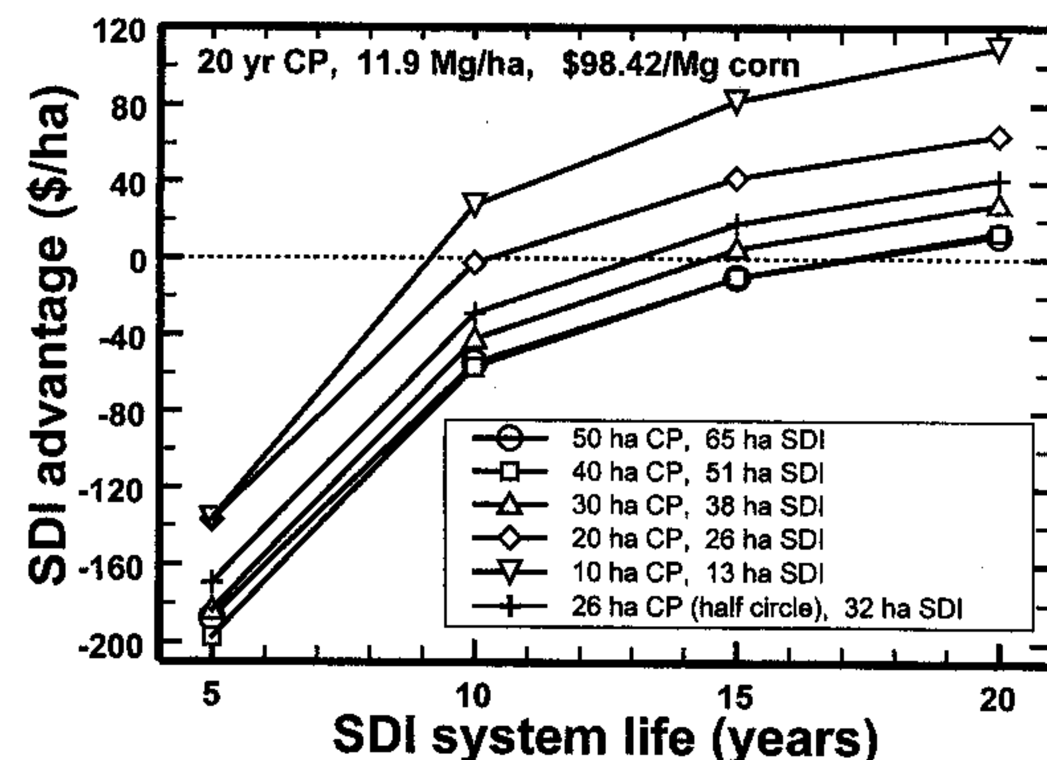
Figure 4—Net returns advantage of SDI over center pivot sprinkler irrigation as affected by system size and SDI life.
