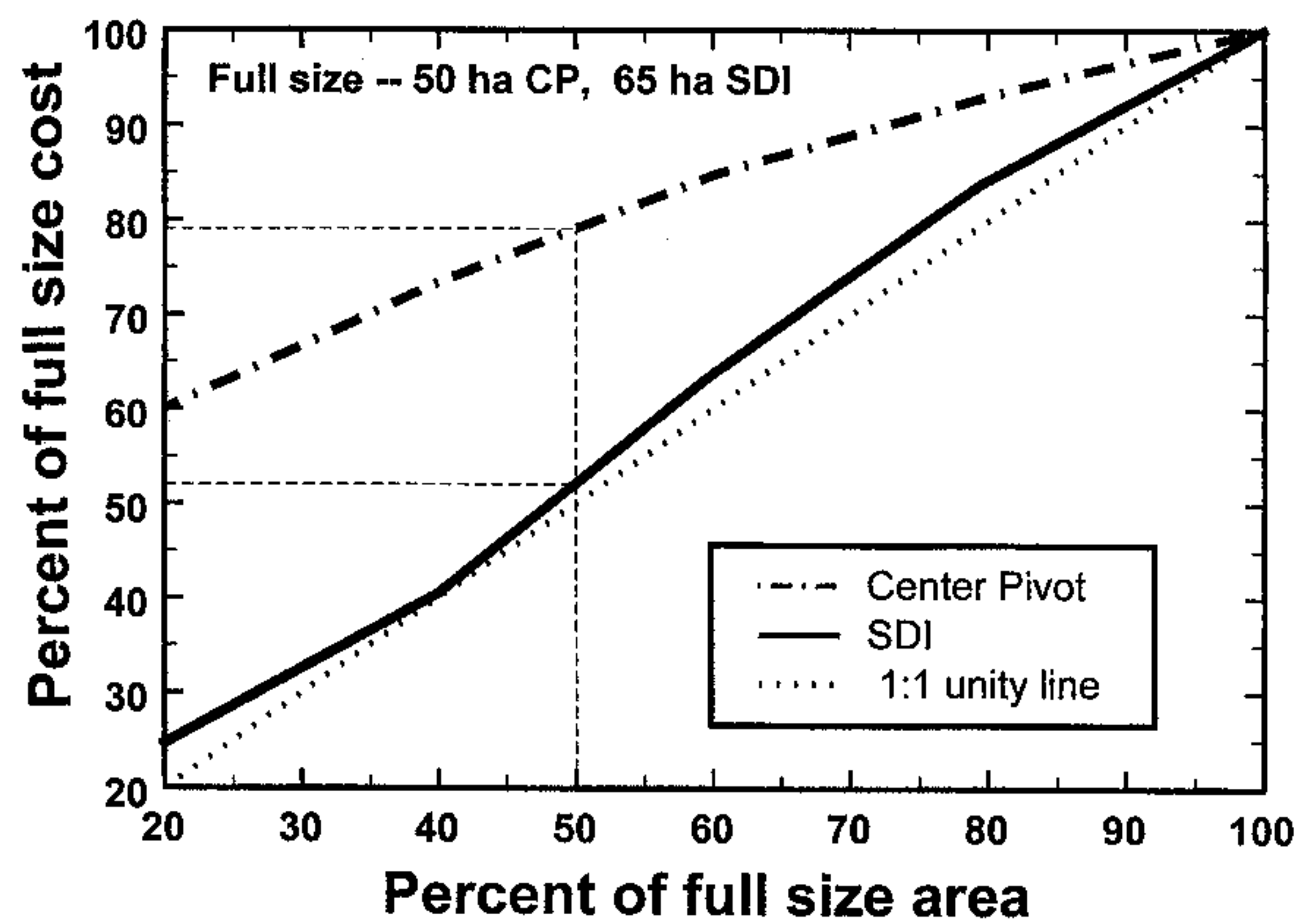
Figure 2—Investment cost as affected by system size for SDI and center pivot sprinkler irrigation systems.
