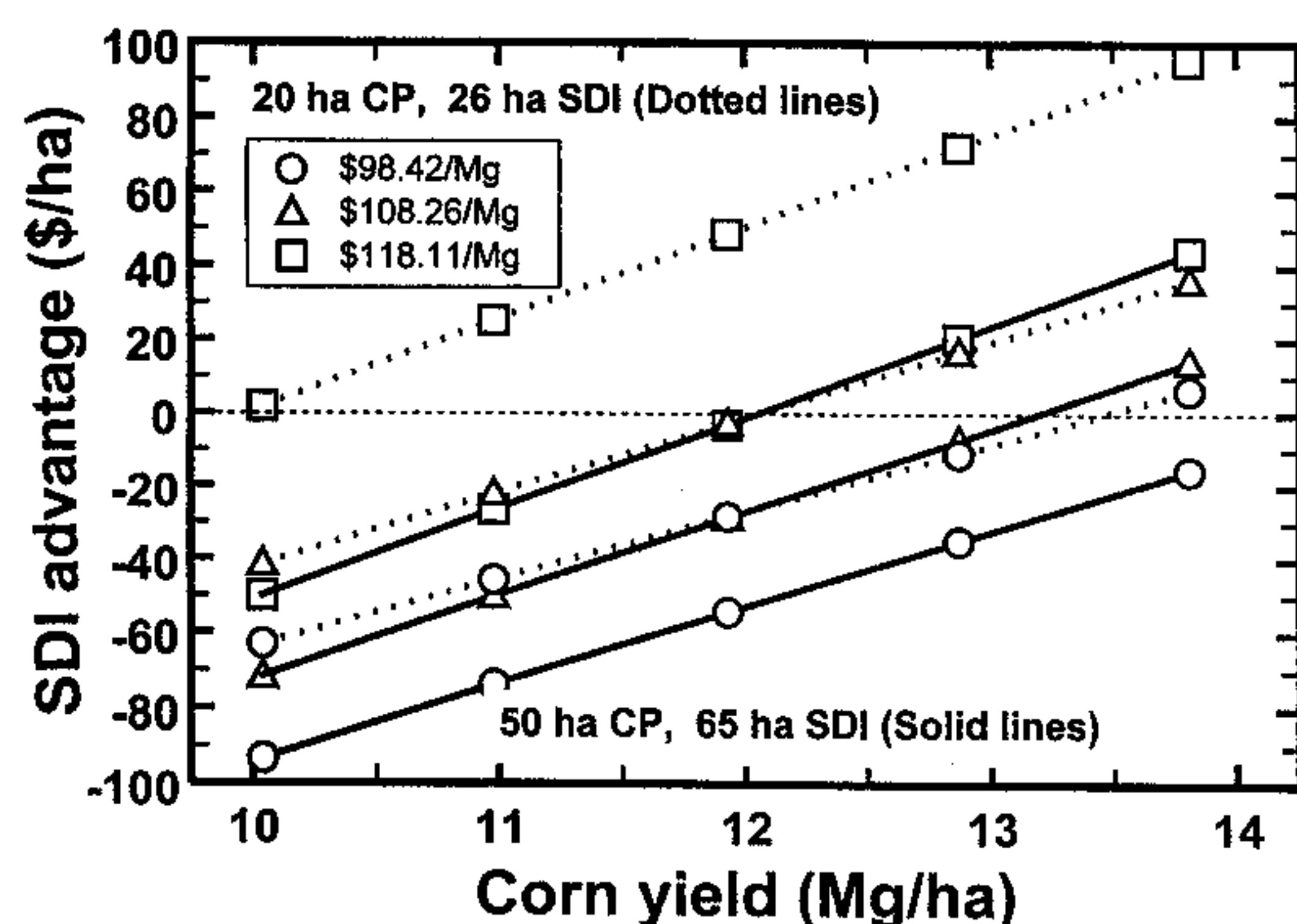
Figure 3—Net returns advantage of SDI over selected center pivot sprinkler irrigation systems as affected by corn yield and price.
