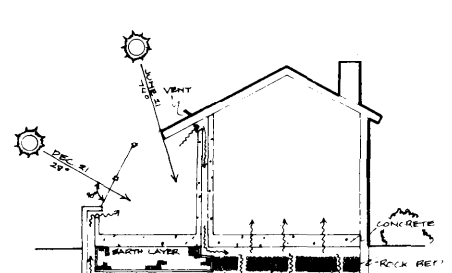
Hot air is forced through the floor and radiates into the house.
