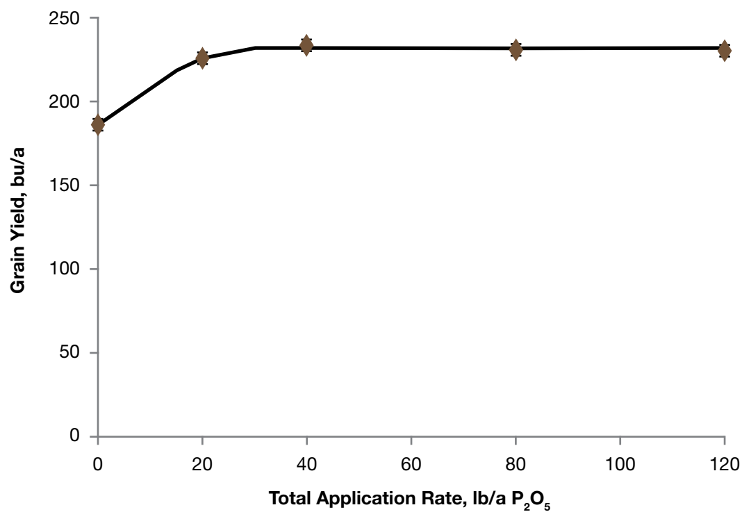
Figure 2. Phosphorus fertilizer application and corn grain yield response at Scandia in 2007 and 2008.
