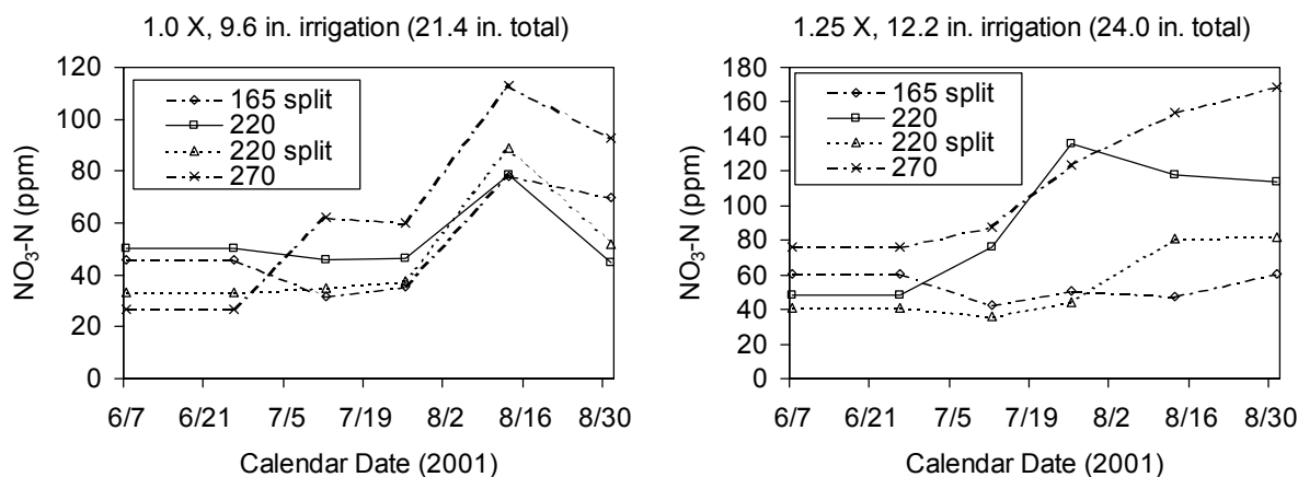
Figure 4. Soil water NO 3 -N concentration at the 60-in. depth collected during the growing season at the Ellinwood site.
