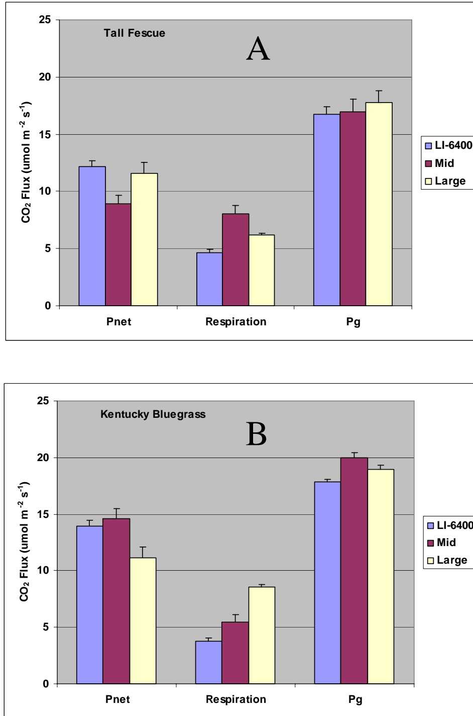
Figure 3. Estimates of net photosynthesis (Pnet), respiration (canopy and soil), and gross photosynthesis (Pg) in tall fescue (A) and Kentucky bluegrass (B). Small chamber is denoted by LI-6400.
