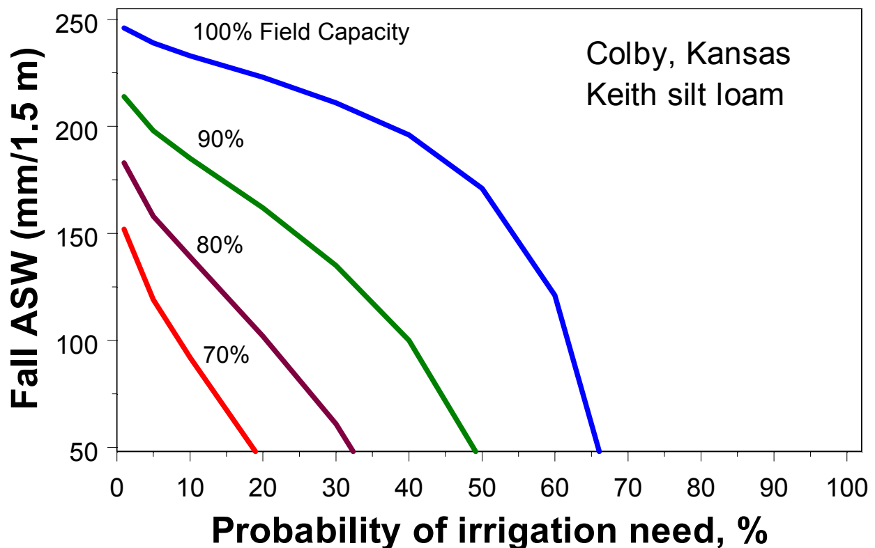
Figure 2. Probability of reaching specified percentage of field capacity by June 1 with a specified value of fall (November-December) available soil water (ASW) in the 1.5-m soil profile on a Keith silt loam soil at Colby, KS. After Lamm and Rogers (1985).
