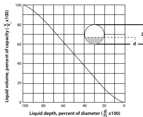
Figure 1. Depth-to-volume relationship for a cylindrical tank.
