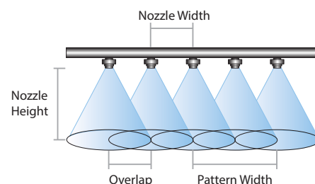
Figure 11. Nozzle overlap of 100 percent.
